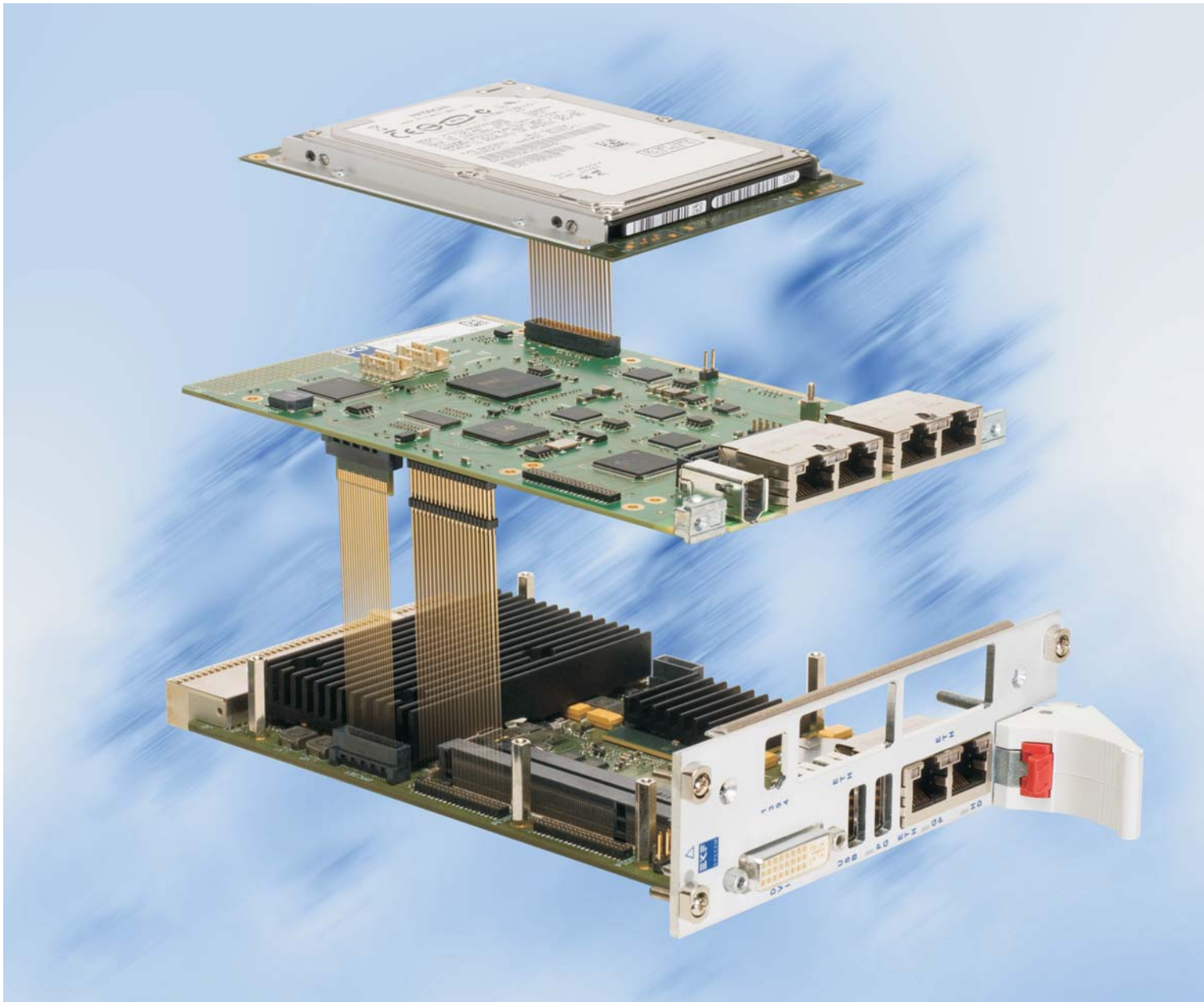
Sample 8HP Mezzanine Assembly (Exploded View)
